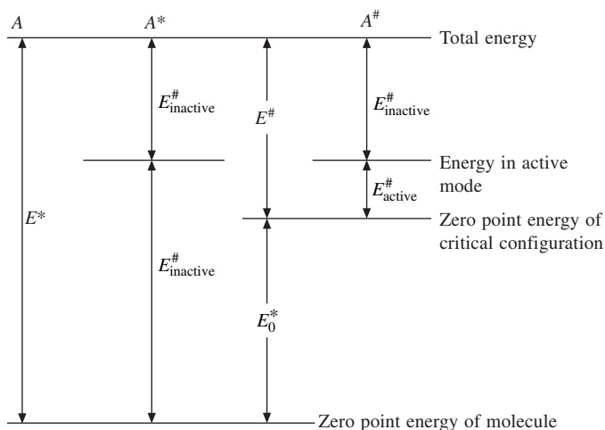
Fig. 4.12 Energy scheme for RRKM theory.
