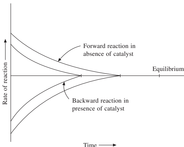
Fig. 6.2 State of equilibrium in absence as well as in presence of a catalyst.
