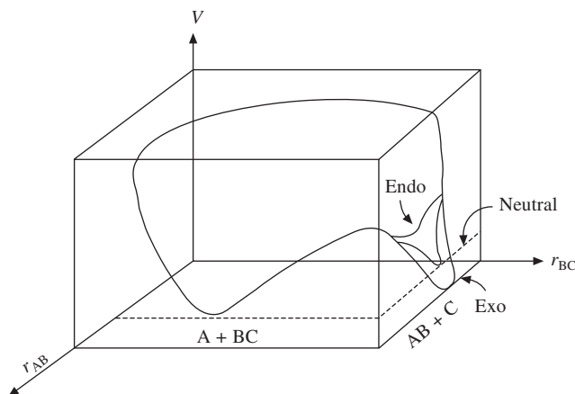
Fig. 9.11 PES for a collinear system A + BC \rightarrow AB + C .
