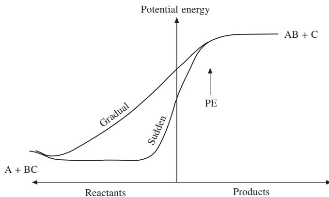
Fig. 9.20 PE profiles for gradual and sudden surfaces.
